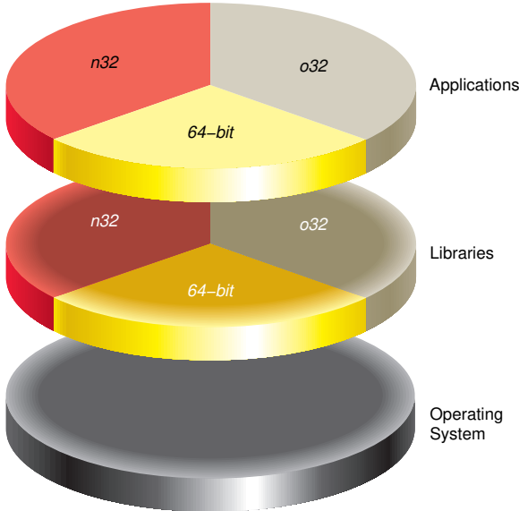
Figure 3-1 Application Support Under Different ABIs
